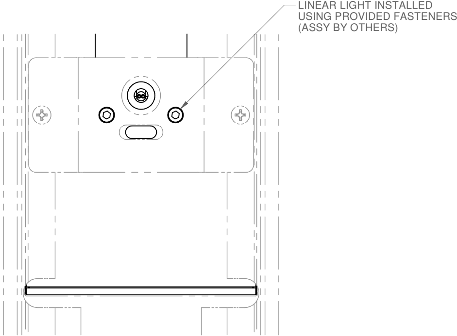
FLUSH CHANNEL TOP VIEW MOUNTING BRACKET DETAIL
