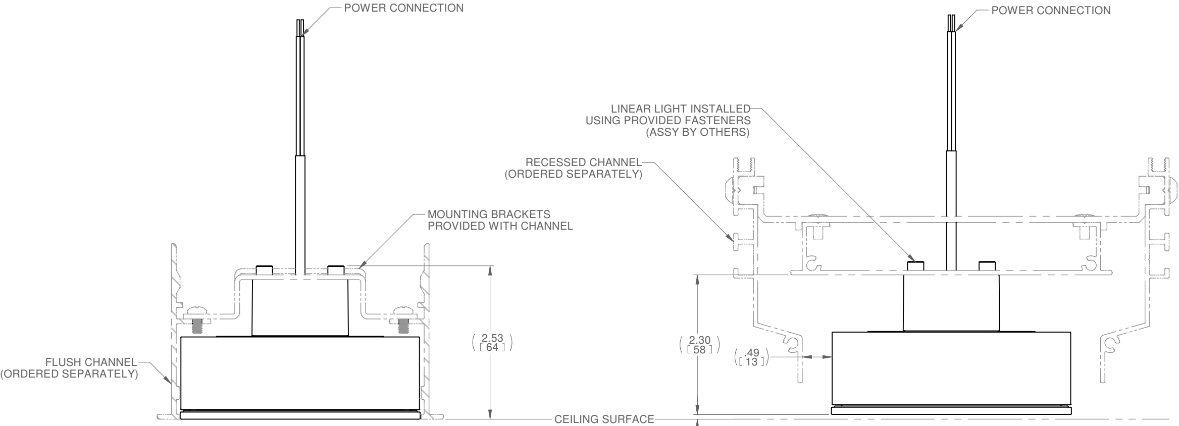
FLUSH CHANNEL END VIEW
